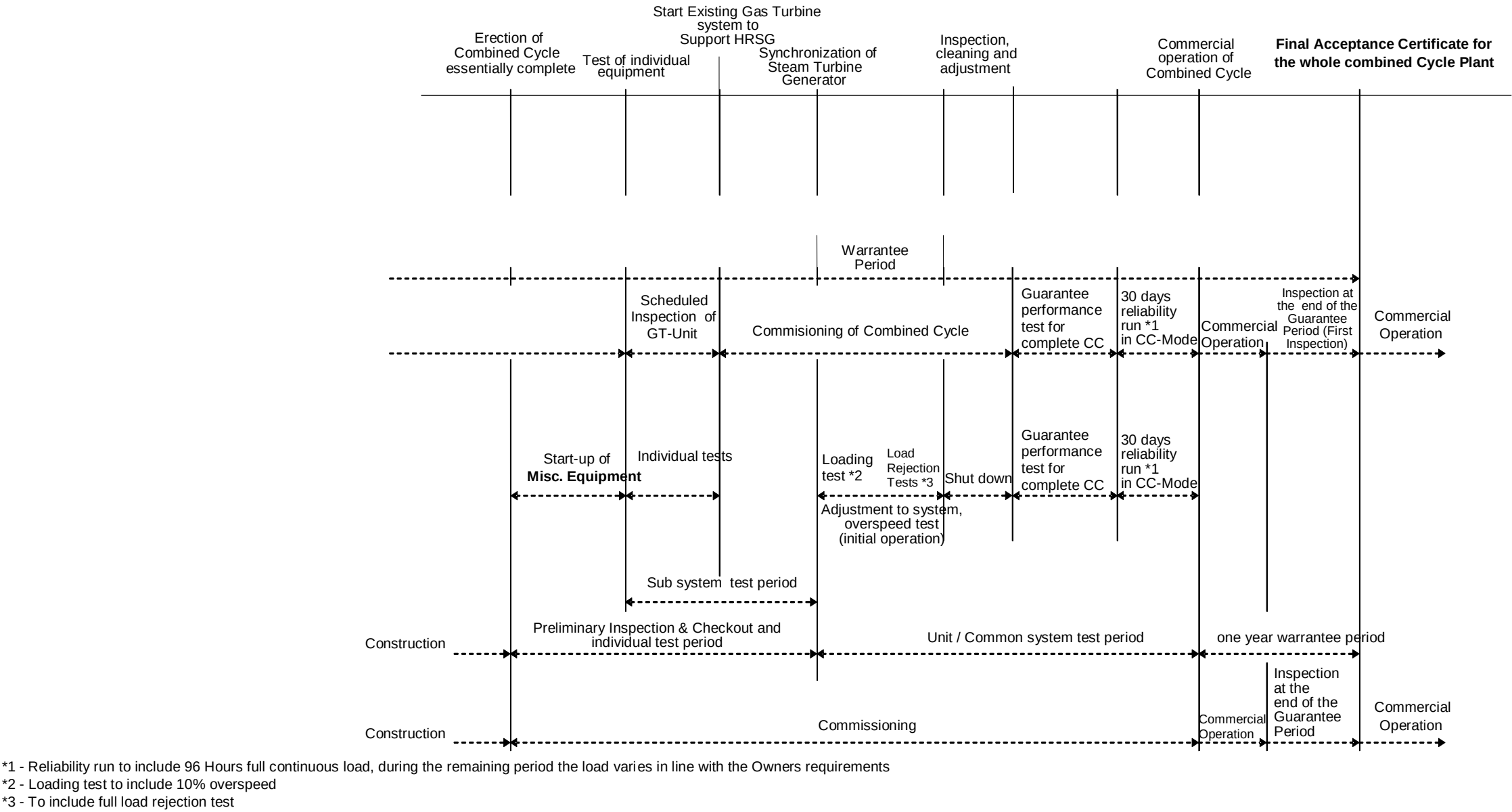
Exhibit 1 Sequence of Events for Start Up and Commissioning for Combined Cycle Block 2, 3 & 4
